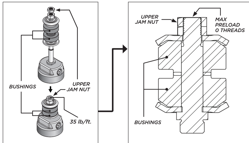
HEAVY DUTY STEM BUSHING DIAGRAM & ASSEMBLY
